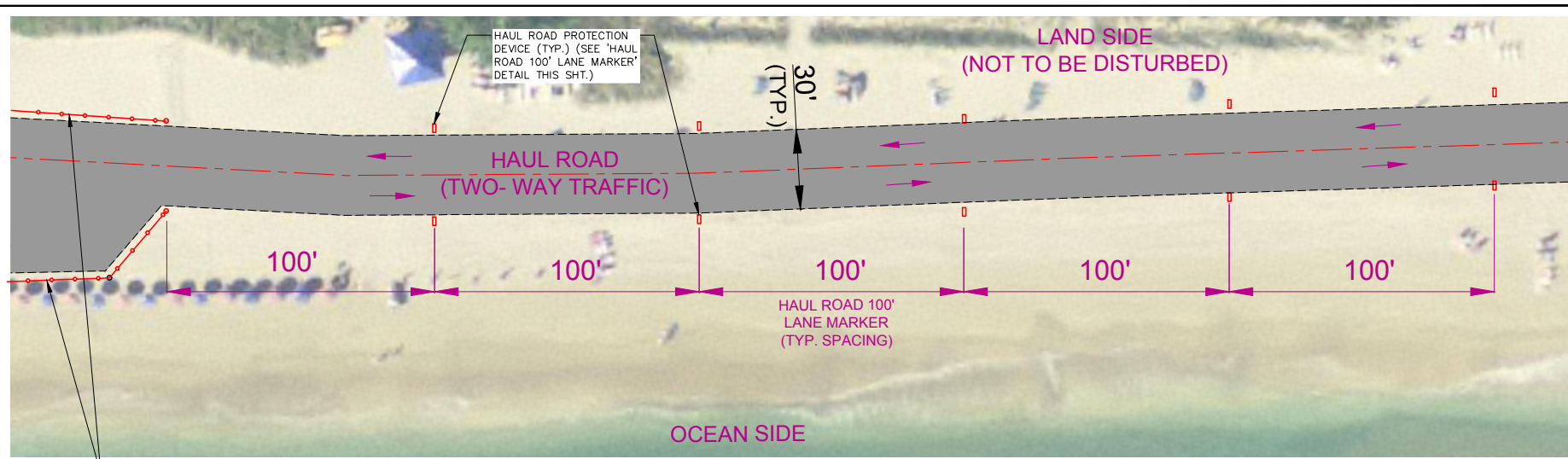
TYPICAL HAUL ROAD TRAFFIC CONTROL LAYOUT PLAN SCALE: 1:20
